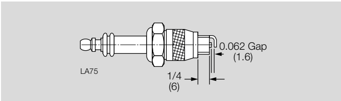
Part number 16160. 10 mm self-grounding igniter.
