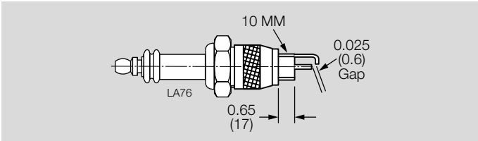
Part number 18458. 10 mm self-grounding igniter.
